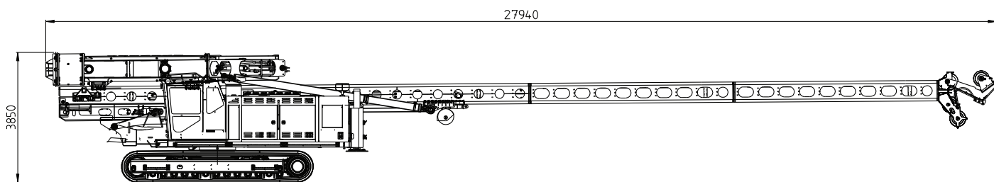
PMx25 transport dimensions with longest available leader configuration (Hydraulic Impact Hammer SHK7).
