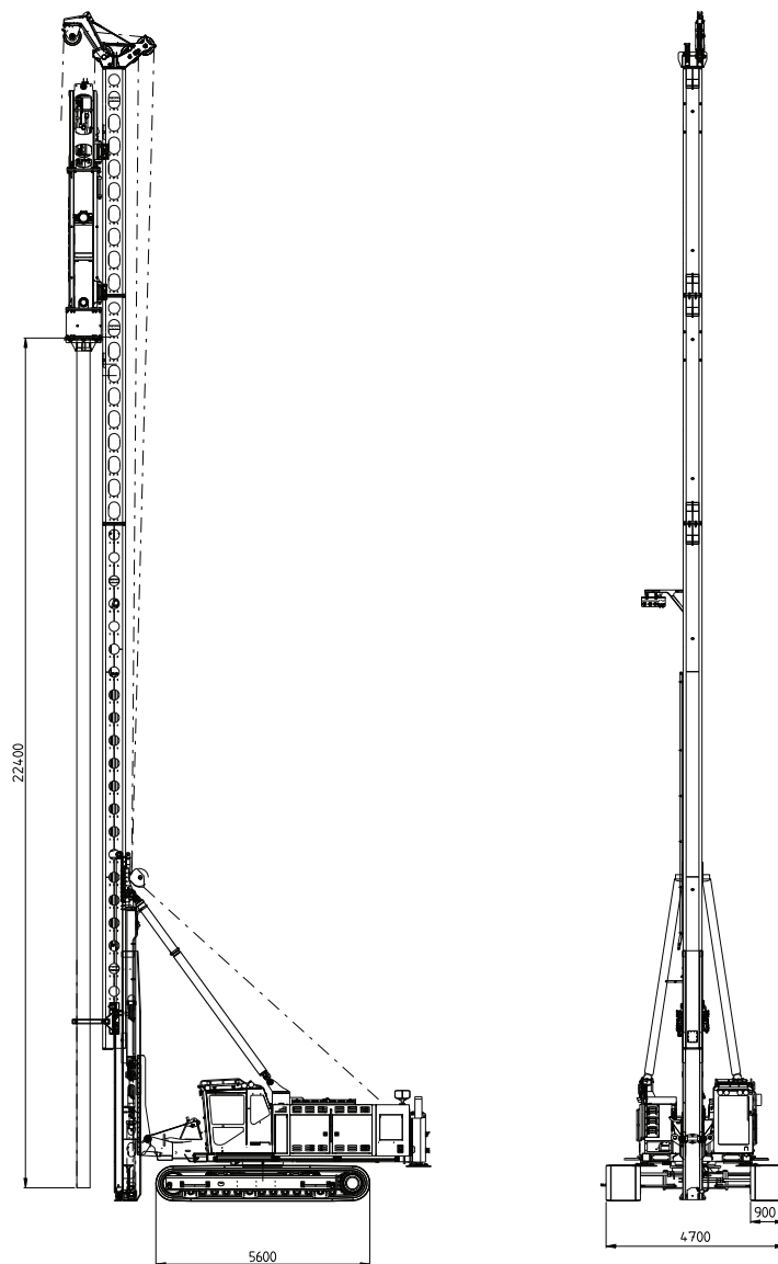
PMx25 with longest available leader configuration (Hydraulic Impact Hammer SHK7)
