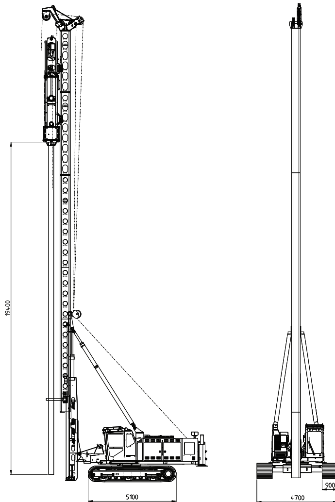
PMx22 with longest available leader configuration (Hydraulic Impact Hammer SHK5)
