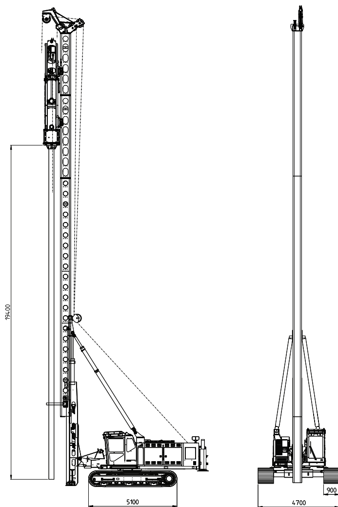
PMx22 with longest available leader configuration (Hydraulic Impact Hammer SHK100-5)
